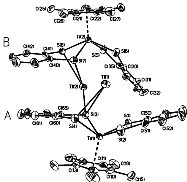
Fig. 2 Perspective view of the two structurally different units of \text{TlTiCp}^*(\text{bdt})_2 1 (30% probability displacement ellipsoids)
